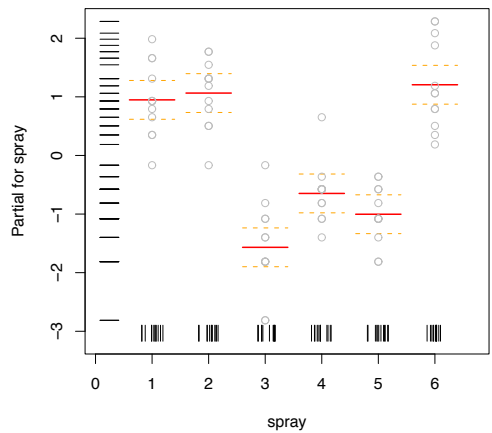
Figure 14: Graphical representation of the results from the function aov with termplot() .
